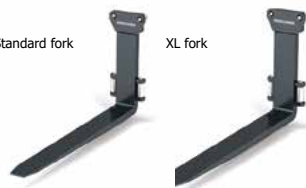
Different cross-sections, lengths, tapering, and reinforcements
